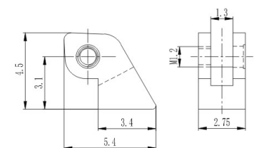
弹簧前铰 Front hinge for metal frame XD7030-27/0
