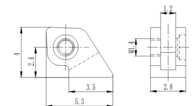
弹簧前铰 Front hinge for metal frame XD7046-28/0
