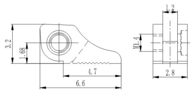
弹簧前铰 Front hinge for metal frame XD706C28/0
