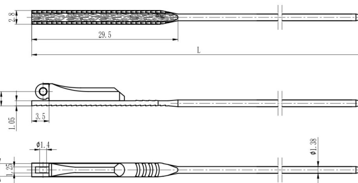
弹簧插芯 Spring hinge wire core
