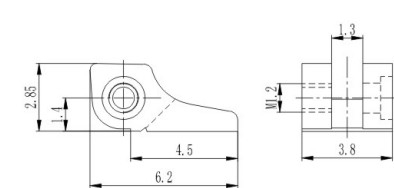
弹簧前铰 Front hinge for metal frame XD7134A38/0
