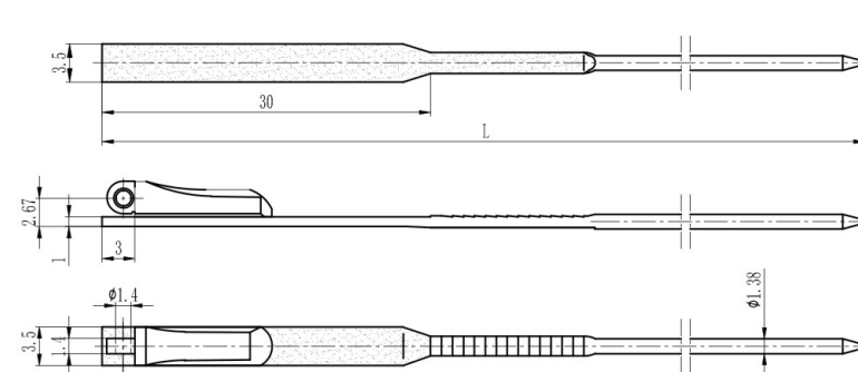
弹簀插芯 Spring hinge wire core
