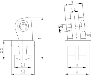
弹簀塑铰 Front hinge for plastic frame XD7014-40/N0
