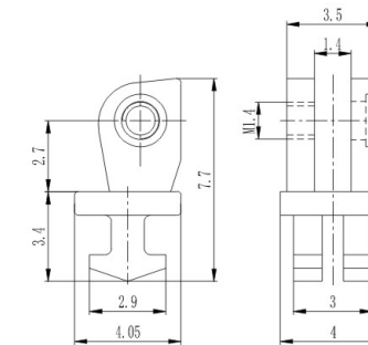
弹簀塑铰 Front hinge for plastic frame XD734E40/N0
