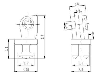
弹簧塑铰 Front hinge for plastic frame XD928H35/N0
