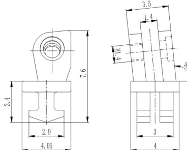
弹簀塑铰 Front hinge for plastic frame XD734-40/N0
