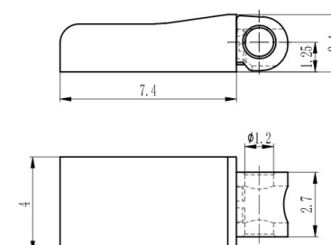
组合弹簧盒 Spring hinge XDF4021A40-Y
