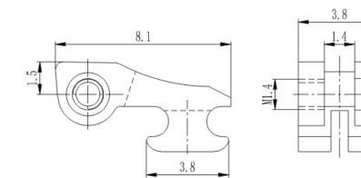
弹簧塑铰 Front hinge for plastic frame XD774-38/N0
