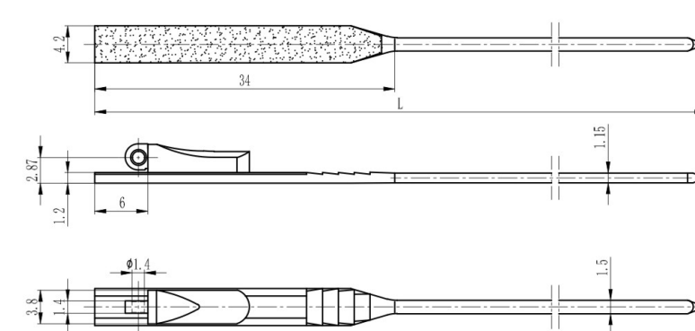
弹簧插芯 Spring hinge wire core
