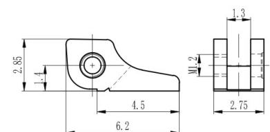
弹簧前铰 Front hinge for metal frame XD7134-27/W
