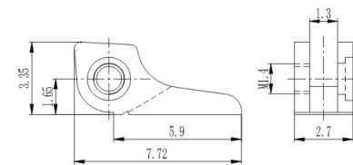
弹簧前铰 Front hinge for metal frame XD984-F27/0
