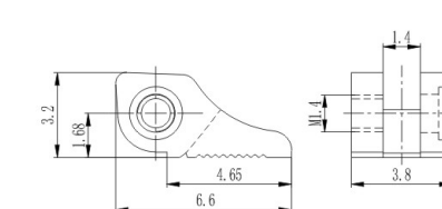
弹簧前铰 Front hinge for metal frame XD706-38/0
