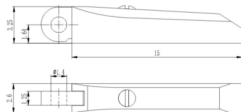
组合弹簧盒 Spring hinge XFP939B26/Y
