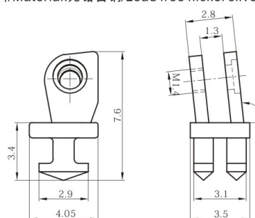
弹簧塑铰 Front hinge for plastic frame XD928H35/N0
