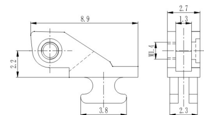
弹簧塑铰 Front hinge for plastic frame XD854-27/N0
