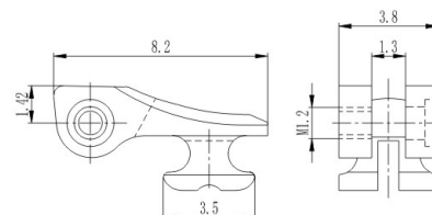
弹簧塑铰 Front hinge for plastic frame XD798B38/N0
