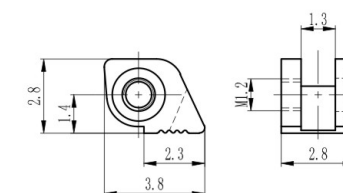
弹簧前铰 Front hinge for metal frame XDA7124A28-W
