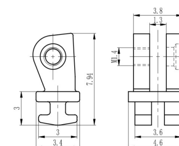
弹簧塑铰 Front hinge for plastic frame XD224-46/WG01
