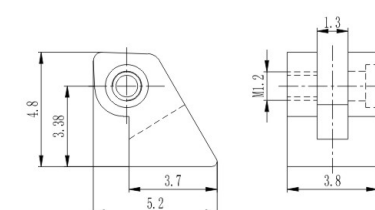
弹簧前铰 Front hinge for metal frame XD014-38/0
