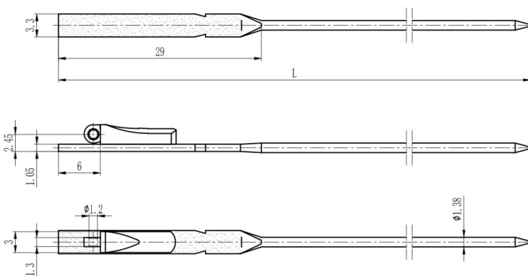
弹簧插芯 Spring hinge wire core
