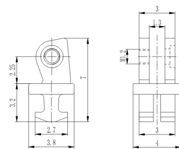
弹簀塑铰 Front hinge for plastic frame XD7014M40/N0
