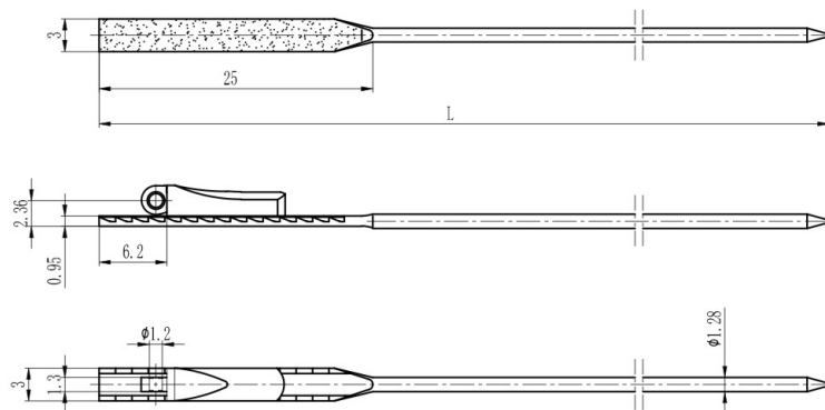
弹簧插芯 Spring hinge wire core
