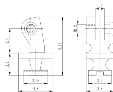
弹簧塑铰 Front hinge for plastic frame XD184-A38/N0
