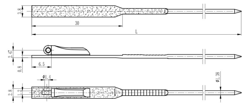
弹簧插芯 Spring hinge wire core
