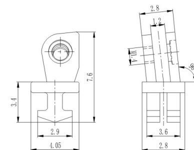
弹簧塑胶 Front hinge for plastic frame XD734-36/N0
