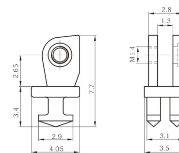
弹簧塑铰 Front hinge for plastic frame XD928-35/N0
