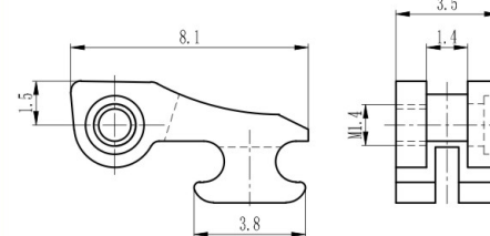
弹簀塑铰 Front hinge for plastic frame XD774-35/N0
