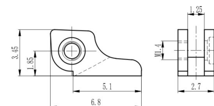
弹簧前铰 Front hinge for metal frame XD918-27/W
