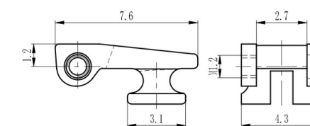
弹簧塑铰 Front hinge for plastic frame XDB4010-43-WN
