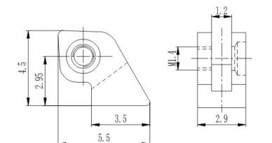
弹簧前铰 Front hinge for metal frame XD754-29/0
