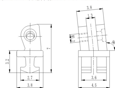
弹簧塑铰 Front hinge for plastic frame XD7014-45/N0
