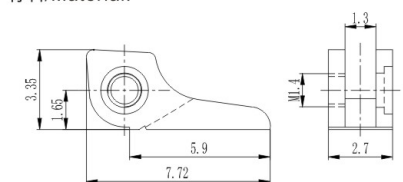
弹簧前铰 Front hinge for metal frame XD984-F27/0
