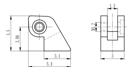
弹簀前铰 Front hinge for metal frame XD7030-30/0
