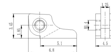
弹簧前铰 Front hinge for metal frame XD918-27/0
