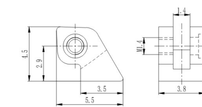
弹簧前铰 Front hinge for metal frame XD754-38/0
