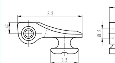
弹簧塑胶 Front hinge for plastic frame XD798-30/N0
