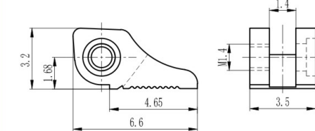
弹簀前铰 Front hinge for metal frame XD706-35/0
