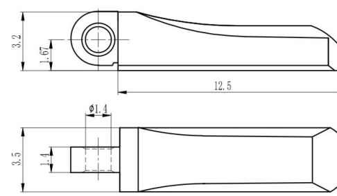
组合弹簀盒 Spring hinge XFP7025-35/0
