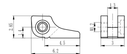
弹簀前铰 Front hinge for metal frame XD7134-30/0
