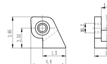
弹簧前铰 Front hinge for metal frame XD7032A30/0
