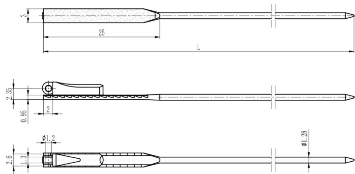
弹簧插芯 Spring hinge wire core
