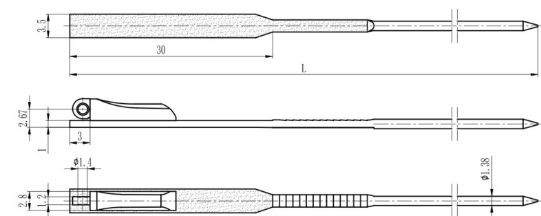
弹簧插芯 Spring hinge wire core
