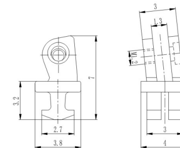
弹簧塑胶 Front hinge for plastic frame XD7014-40/N0
