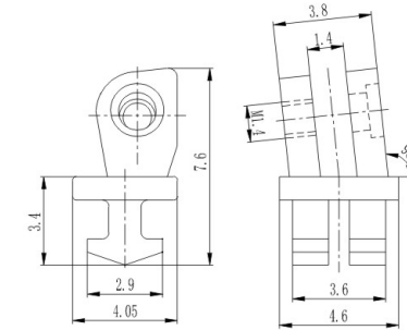
弹簧塑铰 Front hinge for plastic frame XD734-46/N0
