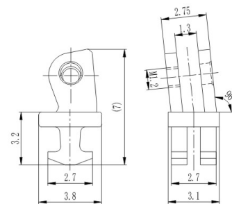
弹簧塑铰 Front hinge for plastic frame XD7014-31/N0
