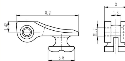
弹簀塑铰 Front hinge for plastic frame XD798-30/N0
