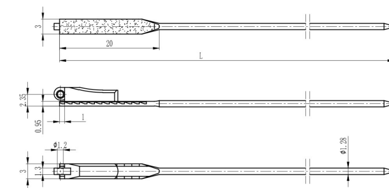
弹簧插芯 Spring hinge wire core
