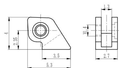
弹簧前铰 Front hinge for metal frame XD8502-F27/0
