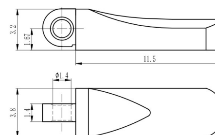
组合弹簧盒 Spring hinge XFP7105-38/0
