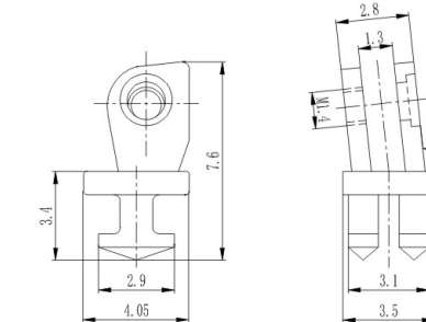
弹簧塑铰 Front hinge for plastic frame XD928H35/N0
