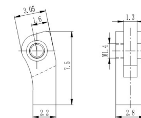
弹簧前铰 Front hinge for metal frame XD054-28/0
