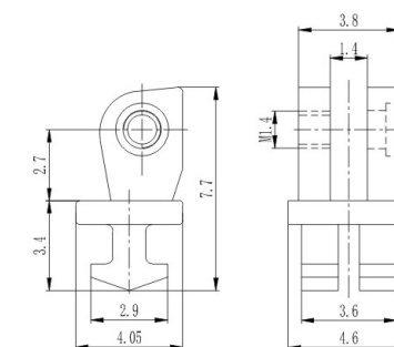
弹簧塑铰 Front hinge for plastic frame XD734C46/N0
