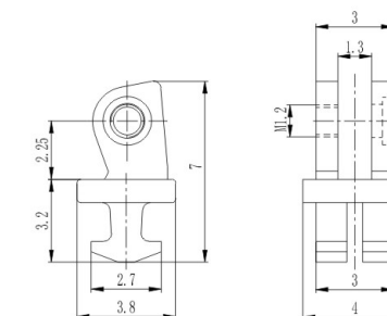
弹簧塑胶 Front hinge for plastic frame XD7014M40/N0
