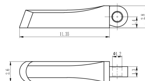
组合弹簧盒 Spring hinge XFP7121-26/W
