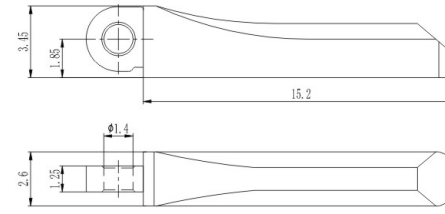
组合弹簧盒 Spring hinge XDF913DA26-Y
