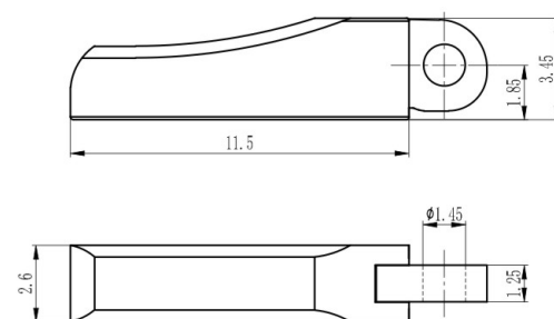
组合弹簧盒 Spring hinge XFP055-26/W
