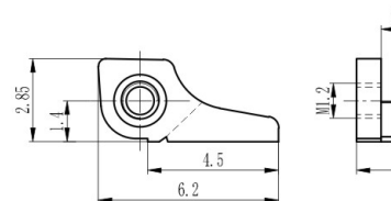
弹簧前铰 Front hinge for metal frame XD7134-30/0
