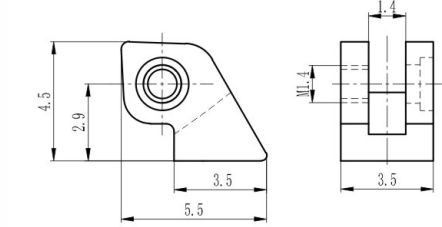
弹簀前铰 Front hinge for metal frame XD754-35/0
