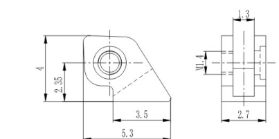
弹簧前铰 Front hinge for metal frame XD8502-F27/0
