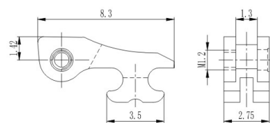
弹簧塑铰 Front hinge for plastic frame XD798-27/N0
