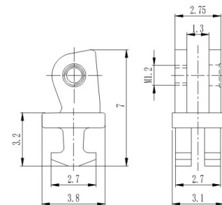
弹簧塑铰 Front hinge for plastic frame XD7014A31/N0
