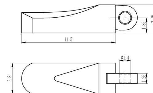
组合弹簧盒 Spring hinge XFP113-38/W
