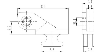
弹簧塑铰 Front hinge for plastic frame XD854-27/N0
