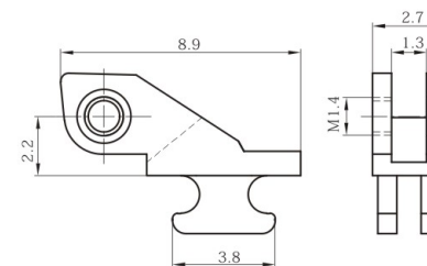
弹簧塑铰 Front hinge for plastic frame XD854-27/N0
