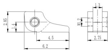
弹簧前铰 Front hinge for metal frame XD7134-27/0
