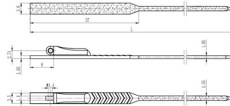
弹簀插芯 Spring hinge wire core
